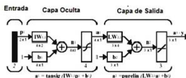
Figura 2. multilayer feed forward back propagation network
