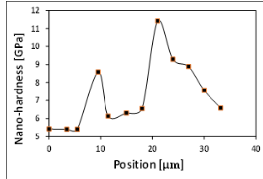
Figure 5. Nano-hardness profile of AISI 316 coated with Al-Si
