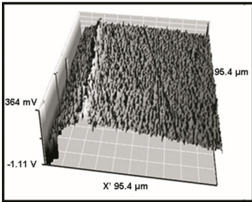
Figure 4. Differential voltage on cross-section of Al-Si coating with TT, after to be oxidized in a water vapor loop at 750°C during 400 hours
