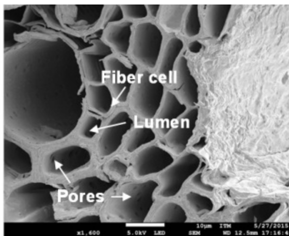
Figure 3. SEM micrographs of untreated pineapple leaf fiber.
