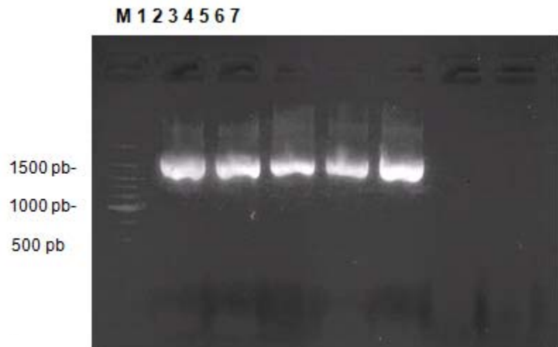
Figure 4. PCR for rDNA 16S gene from Klebsiella species M) Molecular weight marker 100 bp 1) Klebsiella pneumoniae pneumoniae strain PUJ 017 2) Klebsiella pneumoniae ozaenae strain PUJ 040 3) Klebsiella oxytoca 4) Klebsiella pneumoniae rhinoscleromatis -like clinical isolate 5) Klebsiella pneumoniae ozaenae strain PUJ 040 6) DNA control extraction 7) Amplification control.
