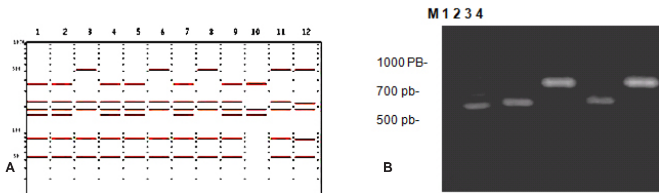
Figure 3. A. In silico prediction of restriction patterns with Taq I for rDNA 16S amplicon from Klebsiella species. Lines: 1, Klebsiella pneumoniae pneumoniae ; 2 to 5 Klebsiella pneumoniae ; 6 to 8 Klebsiella pneumoniae ozaenae ; 9 to 10 Klebsiella pneumoniae rhinoscleromatis ; 11 Klebsiella oxytoca ; 12, Klebsiella granulomatis . B. Restriction of rDNA 16S with Taq I enzyme M) Molecular weight marker 100 bp (Promega) 1) Klebsiella pneumoniae pneumoniae PUJ 017 2) Klebsiella pneumoniae ozaenae PUJ 040 3-4) Klebsiella pneumoniae clinical isolates.
