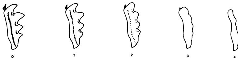
Fig.4. Different categories of tibial wear in termites of Bubas bubalus : from unused (0) to maximum wear (4).
