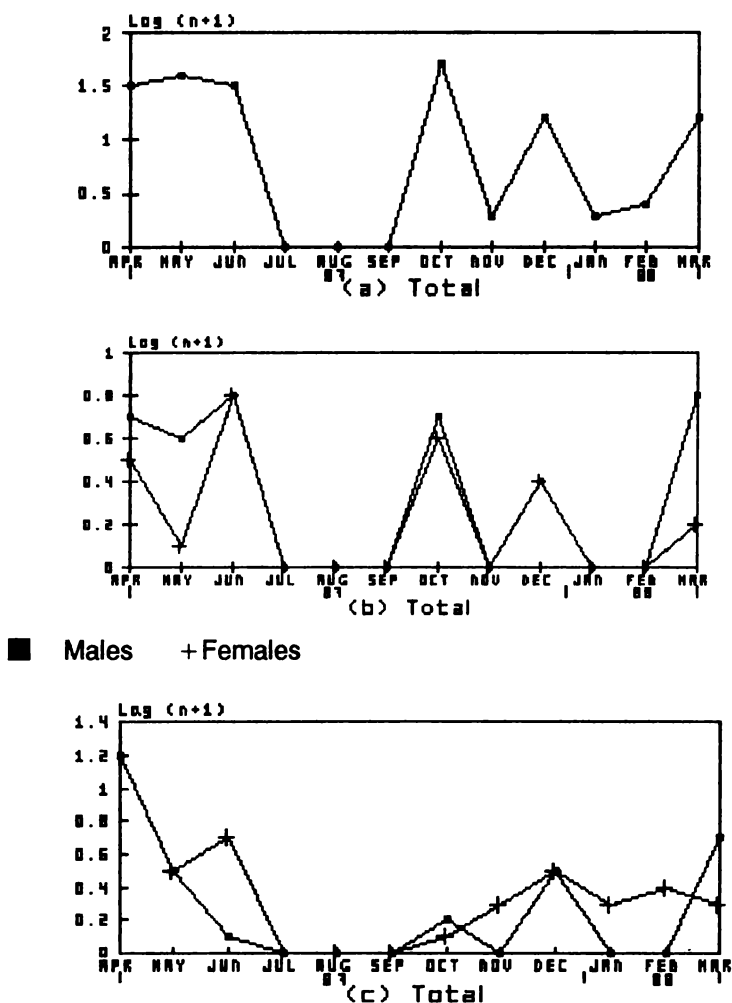
Fig.5. Seasonal activity of adult Bubas bubalus at "Castro Enríquez" from April 1987 to March 1988: (a) total number of beetles caught in traps; (b) trap catches of males and females in a wooded area and (c) in open pasture. n = monthly number of individuals caught in traps.
