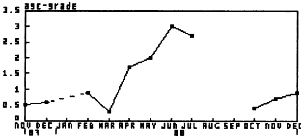
Fig.6. Evolution of the monthly average of age-grade of Bubas bubalus females, based on tibial wear. Due to the difficulty of catching individuals during January, the discontinuous line represents their assumed evolution. m.N = mid-November; f.N. = end of November.
