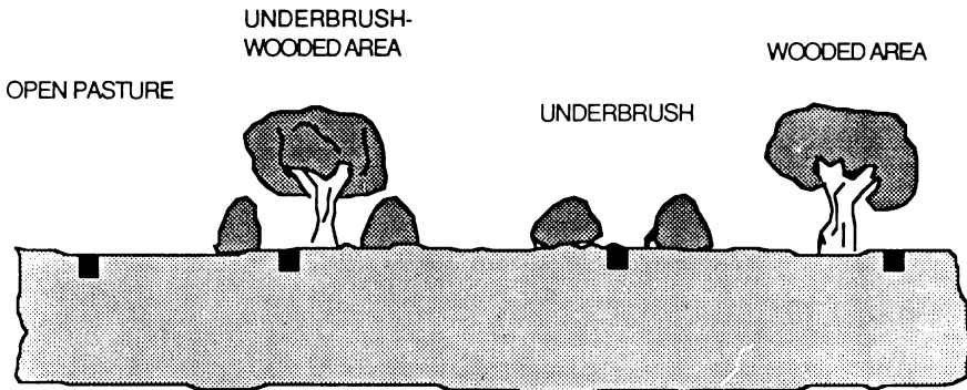
Fig.2. Schematic representation of the diversity of habitats (open pasture, underbrush-wooded area, underbrush and wooded area) and location of the pit-fall traps ■ at "Campillo" (41°0' N and 6°3' W; average altitude of 805 m a.s.l.)
