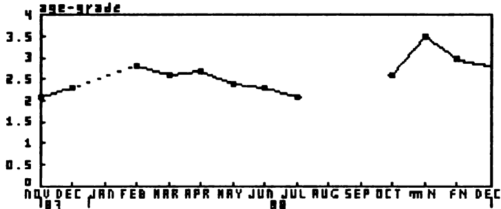
Fig.9. Evolution of the monthly average of fat-body accumulation in the abdomen of Bubas bubalus females, taking into consideration 5 categories (from 0 to 4) of lesser to greater abundance. Due to the difficulty of catching individuals during January, the discontinuous line represents the assumed evolution. m.N. = mid-November; f.N. = end of November.
