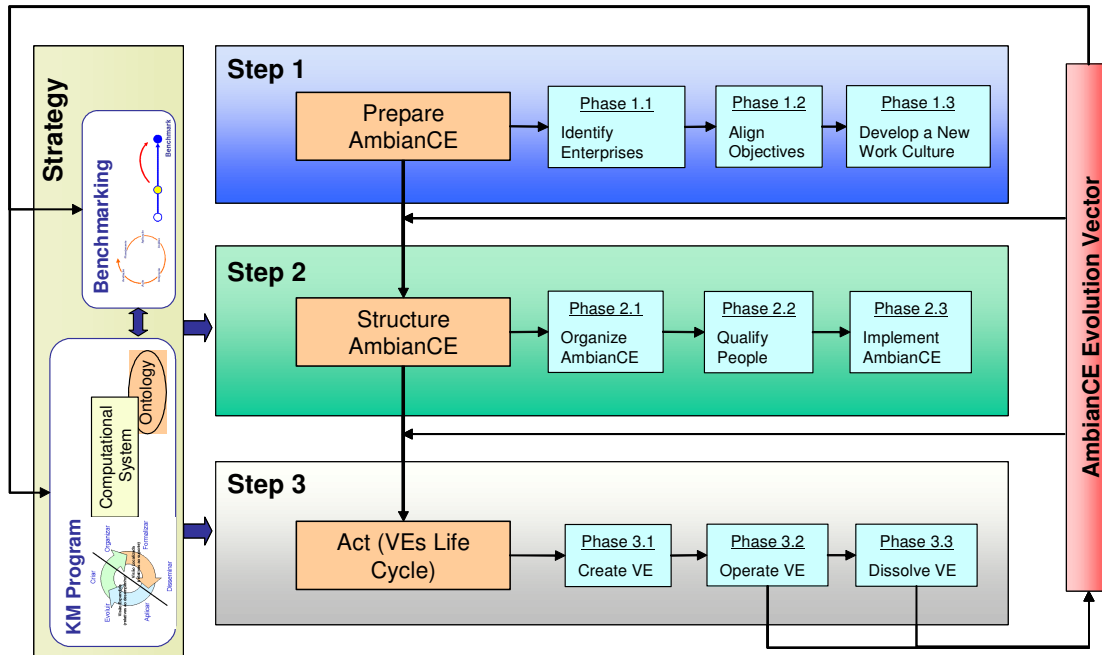
Figure 1: AmbianCE framework and its constitutive elements.
