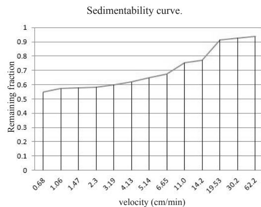
Figure 2. Sedimentability curve.
