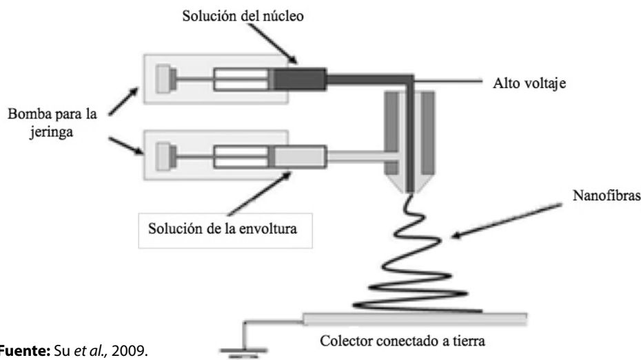
Figura 2. Esquema general de la disposición y procesos de electrohilado co-axial Figure 2. General schematic of the arrangement and process of co-axial electrospinning.
