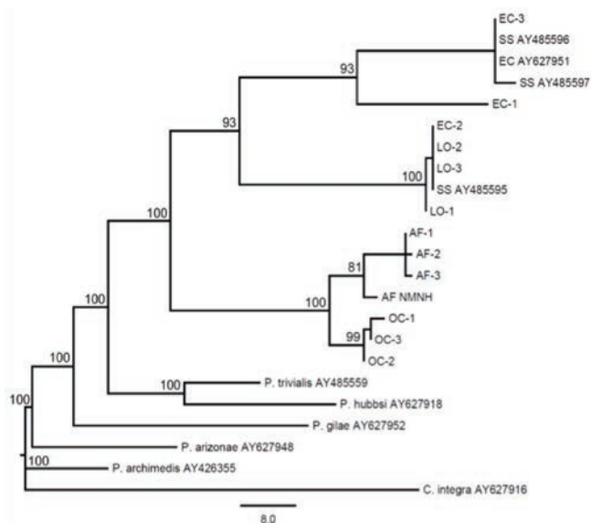
Figure 2. Maximum parsimony phylogenetic tree of specimens of P. bernardina and other closely related taxa using a fragment of the COI gene (578 bp). SS (Snail Spring; GenBank specimens SS AY485595, SS AY485596 and SS AY485597); EC (El Chorro; GenBank specimen AY627951); LO (Los Ojitos); AF (Agua Fria); OC (Ojo Caliente). Numbers above nodes indicate statistical support
