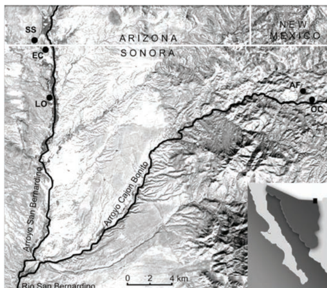
Figure 1. General location of study area in southeastern Arizona and northeastern Sonora. Black spots indicate sampling sites of the Sonoran populations of Pyrgulopsis bernardina in the San Bernardino River drainage. Snail Spring = SS, El Chorro = EC, Los Ojitos = LO, Agua Fria = AF, Ojo Caliente = OC, San Bernardino National Wildlife Refuge = SBNWR
