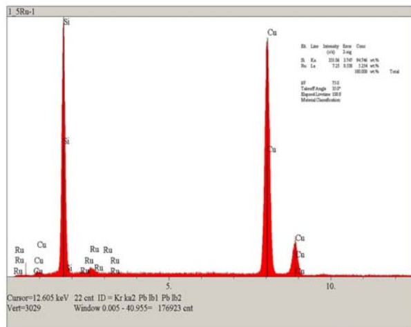
Figure 4. EDX spectrum catalyst Ru/SiO 2 1,5%
