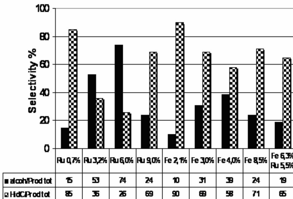
Fig. 10. Fischer-Tropsch reaction selectivity from supported ruthenium, iron and bimetallic Fe/Ru catalysts.
