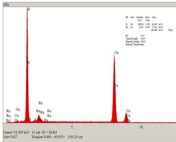
Figure 2. EDX spectrum for catalyst Ru/SiO 2 6%
