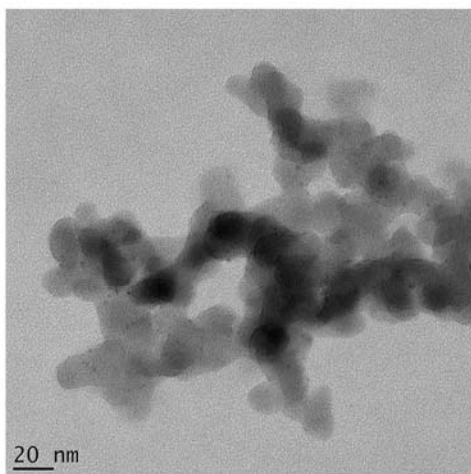
Figure 3. TEM photo of silica-supported 1,5 % Ru nanoparticle
