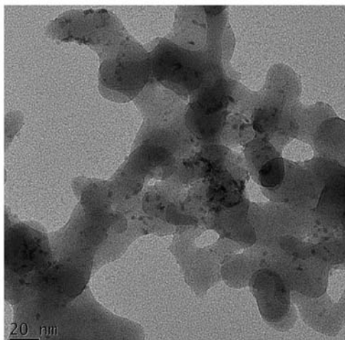
Figure 1. TEM photo of silica-supported Ru nanoparticles 6%
