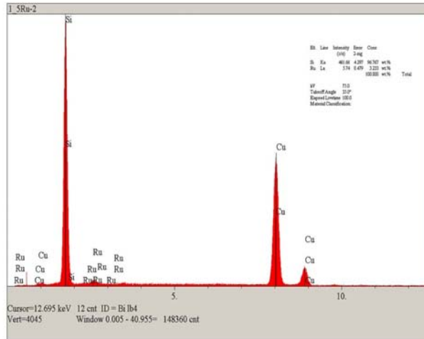
Figure 6. EDX spectrum catalyst Ru/SiO 2 1,5%
